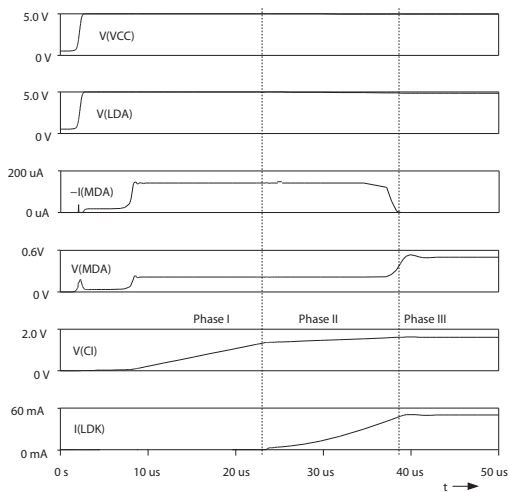
Figure 1: Turn-on behaviour
