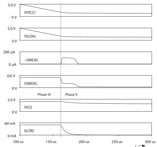
Figure 2: Turn-off behaviour
